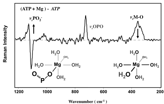
FIGURE 4: Inner-sphere coordination induces \nu_s\text{PO}_2^- \text{M} formation and \nu_s\text{M-O} attenuation. Raman difference spectrum of ATP (60 mM) in the presence of excess MgCl _2 (200 mM), indicating the relative positions of the Mg ^{2+} -induced changes in \nu_s\text{PO}_2^- ( \sim 1100 \text{ cm}^{-1} ) and magnesium hexahydrate ( \nu_s\text{M-O} , 360 \text{ cm}^{-1} , structure at the right). Black arrows reflect previously observed correlations of Mg ^{2+} binding (structure at the left) with an increased \nu_s\text{PO}_2^- inflection and a decreased \nu_s\text{M-O} intensity in DMP solution studies and crystals of the HDV ribozyme (12).
