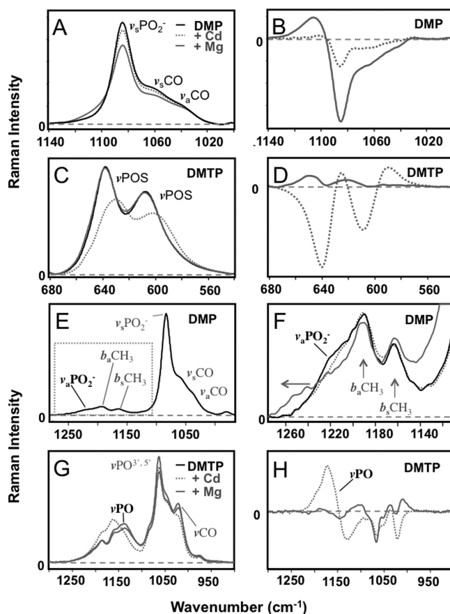
FIGURE 3: Dependence of \nu_s\text{PO}_2^- \text{M} on direct metal ion coordination. (A) Raman spectrum ( 1140\text{--}1000\text{ cm}^{-1} ) of \nu_s\text{PO}_2^- from 0.2 M DMP in the absence of metal (black) or presence of 1 M \text{Mg}^{2+} (gray dots) or 1 M \text{Cd}^{2+} (gray line). (B) Difference spectrum subtracting DMP in the absence of metal from that in the presence of 1 M \text{Mg}^{2+} (gray line) or 1 M \text{Cd}^{2+} (dark gray). (C) Raman spectrum ( 680\text{--}540\text{ cm}^{-1} ) of isolated \nu\text{POS}^- from 0.2 M DMTP in the absence of metal (black) or presence of 1 M \text{Mg}^{2+} (light gray) or 1 M \text{Cd}^{2+} (dark gray). (D) Difference spectrum subtracting DMTP in the absence of metal from that in the presence of \text{Mg}^{2+} (light gray) or 1 M \text{Cd}^{2+} (dark gray). (E) Raman spectrum ( 1300\text{--}950\text{ cm}^{-1} ) showing both symmetric ( \nu_s\text{PO}_2^- ) and asymmetric ( \nu_a\text{PO}_2^- ) stretches for nonbridging phosphate oxygens from 0.2 M DMP in the absence of metal (black) or presence of 1 M \text{Mg}^{2+} (light gray) or 1 M \text{Cd}^{2+} (dark gray). (F) Enlargement of the region of the Raman spectrum shown as a dotted box in panel E showing DMP in the absence of metal ion (black) or in the presence of 1 M \text{Mg}^{2+} (light gray) or 1 M \text{Cd}^{2+} (dark gray). The assignments of \nu_s\text{PO}_2^- , \nu\text{POS}^- , and \nu\text{PO} have been previously established in the literature (27, 43), and their associated metal-dependent shifts were confirmed by ^{18}\text{O} substitution (data not shown). (G) Raman spectrum ( 1300\text{--}900\text{ cm}^{-1} ) near the phosphoryl vibrational mode ( \nu\text{PO} ) from 0.2 M DMTP in the absence of metal (black) or presence of 1 M \text{Mg}^{2+} (light gray) or 1 M \text{Cd}^{2+} (light gray). Additional peaks of bridging \text{O--P--O} ( \nu\text{PO}_3^{3-} ) and \text{C--O} stretch ( \nu\text{CO} ) are shown for reference. (H) Difference spectrum of the region shown in panel G subtracting DMTP in the absence of metal from that in the presence of 1 M \text{Mg}^{2+} (light gray) or 1 M \text{Cd}^{2+} (dark gray). Additional vibrational modes in DMP and DMTP are provided for reference: \nu_s\text{CO} and \nu_a\text{CO} reflect the symmetric and asymmetric \text{C--O} stretch, respectively, and b_s\text{CH}_3 and b_a\text{CH}_3 reflect the symmetric and asymmetric bending modes of the methyl group, respectively (27, 43).
