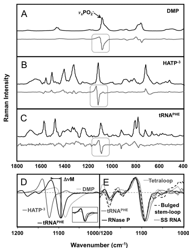
FIGURE 1: Effect of \text{Mg}^{2+} on the Raman spectra of structurally distinct phosphodiesters. Raman spectral data (black) and Raman difference spectra (subtracting spectra at 0\text{ M} from 0.3\text{ M} \text{MgCl}_2 , dark gray) for 200\text{ mM} DMP (A), 100\text{ mM} \text{HATP}^{3-} (B), and 0.81\text{ mM} ( 20\text{ mg/mL} ) yeast \text{tRNA}^{\text{PHE}} (C). (D) Overlay of \text{Mg}^{2+} difference spectra ( 1200\text{--}1000\text{ cm}^{-1} ) of the symmetric stretch for nonbridging phosphate oxygens ( \nu_s\text{PO}_2^- ) for DMP (gray dots), \text{HATP}^{3-} (gray line), and yeast \text{tRNA}^{\text{PHE}} (black). The arrow indicates the spectral distance between inflection points of the positive and negative nodes (marked by vertical black lines) of the \text{Mg}^{2+} -induced inflection of \nu_s\text{PO}_2^- , which defines \Delta\nu\text{M} . The inset shows a superposition of the metal-induced inflections shown in panel D to illustrate the relative similarity in the apparent shift of \nu_s\text{PO}_2^- to higher wavenumbers. (E) Overlay of \text{Mg}^{2+} difference spectra ( 1200\text{--}1000\text{ cm}^{-1} ) of \nu_s\text{PO}_2^- for an 11-nucleotide single-stranded RNA (black dots), 12-nucleotide GAAA tetraloop (gray dots), 27-nucleotide bulged stem-loop sequence (black dashes), 76-nucleotide yeast \text{tRNA}^{\text{PHE}} (dark gray line), and 400-nucleotide E. coli RNase P RNA (black line). Dotted gray boxes indicate the metal-induced inflection of \nu_s\text{PO}_2^- observed in difference spectra. DMP and RNAs were measured at pH 6 ( 200\text{ mM} cacodylate), while \text{HATP}^{3-} was measured at pH 3.8 ( 200\text{ mM} formate) to generate a single negative charge on the terminal phosphate.
