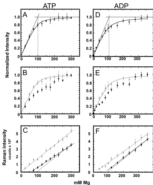
FIGURE 5: Use of \nu_s\text{PO}_2^-\text{M}^{\text{PN}} to monitor site-specific metal ion binding. (A) Dependence of 100 mM protonated ATP ( \text{HATP}^{3-} ) \nu_s\text{PO}_2^-\text{M}^{\text{PN}} on \text{MgCl}_2 concentration (millimolar). Black circles reflect the normalized upshifted \nu_s\text{PO}_2^-\text{M}^{\text{PN}} Raman signal (photon counts) derived from the positive node of the Raman difference spectra ( \nu_s\text{PO}_2^-\text{M}^{\text{PN}} ). The black curve reflects the fit of \nu_s\text{PO}_2^-\text{M}^{\text{PN}} data to the binding isotherm appropriate for approximately equal concentrations of \text{HATP}^{3-} and \text{MgCl}_2 (see Methods). Solid black lines reflect tangents to the initial and saturating phases of the binding curve. The dotted black line reveals the \text{MgCl}_2 concentration corresponding to the intersection of tangent lines above and the stoichiometry of \text{Mg}^{2+} binding to \text{HATP}^{3-} . (B) Dependence of the \text{HATP}^{3-} adenine Raman peak at 1310\text{ cm}^{-1} ( \nu_{\text{A}1310} ) on \text{MgCl}_2 concentration. Black squares reflect the normalized upshifted \nu_{\text{A}1310} Raman signal derived from the positive node of the Raman difference spectra ( \nu_{\text{A}1310}^{\text{PN}} ). The gray ovals and curve reflect the normalized \text{Mg}^{2+} dependence of the increase in \nu_{\text{PO}_2^-\text{M}^{\text{PN}}} as described for panel A. (C) Dependence of the Raman peak for fully hydrated \text{Mg}^{2+} [ \text{Mg}(\text{H}_2\text{O})_6^{2+} , \nu_{\text{Mg-O}} , 360\text{ cm}^{-1} ] on \text{Mg}^{2+} concentration in the absence (gray) and presence of 100 mM \text{HATP}^{3-} (black). Solid lines reflect the linear least-squares fit to all points in the absence (gray) or presence (black) of \text{HATP}^{3-} . Dotted lines reflect the least-squares fit to points above 200 mM \text{MgCl}_2 , where \text{Mg}^{2+} binding to \text{HATP}^{3-} is observed to be saturating. (D–F) Repeats of experiments depicted in panels A–C, respectively, but in the presence of 100 mM protonated ADP ( \text{HADP}^{2-} ). Protonated forms of ATP and ADP were chosen to parallel the single negative charge per phosphate of the other phosphodiester compared in this work.
